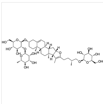
Structure Protopogracillin, CAS 78229-03-5
