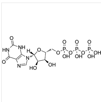
Structure Xanthosine-5'-Triphosphate, CAS 6253-56-1
