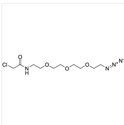
Structure Azido-PEG3-chloroacetamide, CAS 604766-23-6
