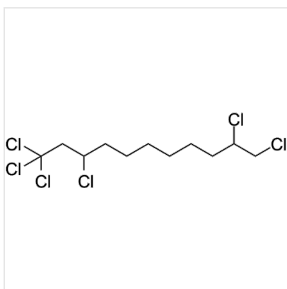
Structure 1,1,1,3,10,11-Hexachloroundecane, CAS 601523-28-8
