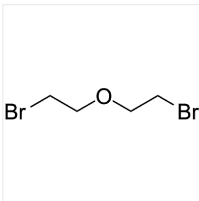
Structure Bis(2-bromoethyl) ether, CAS 5414-19-7
