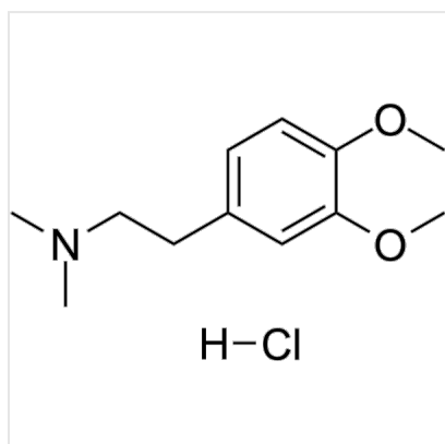
Structure Verapamil EP Impurity C hydrochloride, CAS 51012-67-0
