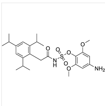
Structure ACAT-IN-3, CAS 454203-25-9
