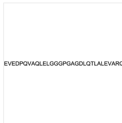
Structure C-Peptide 2, rat, CAS 41594-08-5
