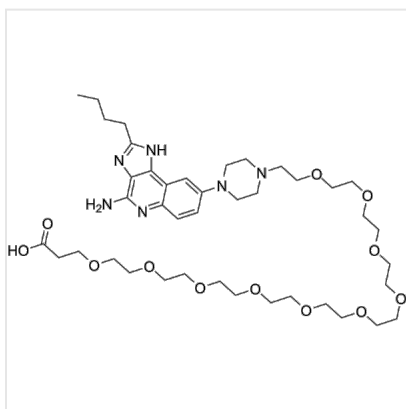
Structure TLR7/8 agonist 4 hydroxy-PEG10-acid, CAS 2388520-17-8
