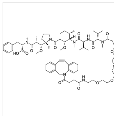
Structure DBCO-PEG4-MMAF, CAS 2360411-65-8
