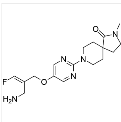
Structure SSAO inhibitor-1, CAS 2242883-04-9
