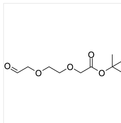
Structure CHO-CH 2 -PEG 1 -CH 2 -Boc, CAS 2230956-95-1
