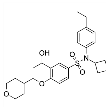
Structure RORgamma inverse agonist 23, CAS 2230779-18-5
