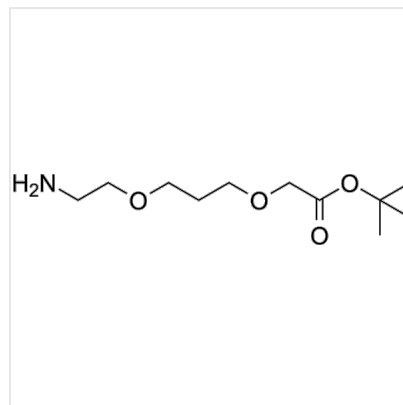
Structure NH2-PEG2-CH2-Boc, CAS 1948273-09-3
