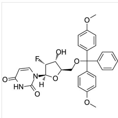
Structure 2'-Deoxy-5'-O-DMT-2'-fluorouridine, CAS 146954-74-7
