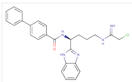
Structure BB-CI-Amidine, CAS 1802637-39-3
