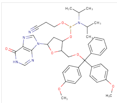
Structure DMT-di Phosphoramidite, CAS 141684-35-7
