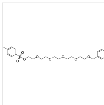
Structure Benzyl-PEG5-Ots, CAS 129086-10-8
