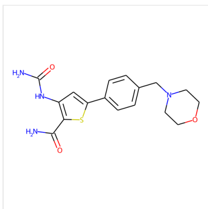
Structure CAY10657, CAS 494772-86-0
