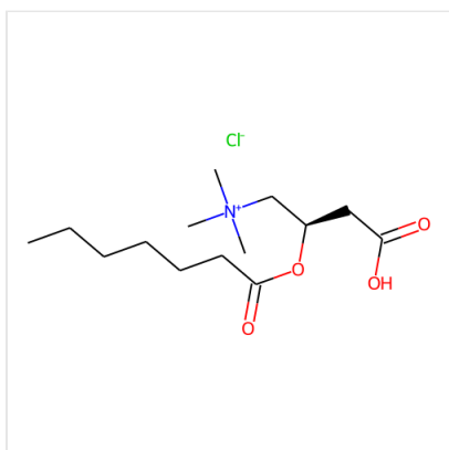
Structure Heptanoyl-L-carnitine (chloride), CAS 162041-08-9
