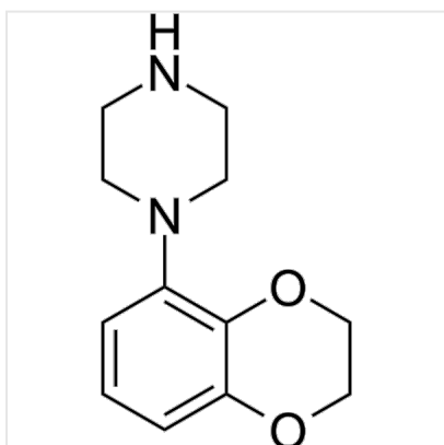
Structure Eltoprazine, CAS 98224-03-4
