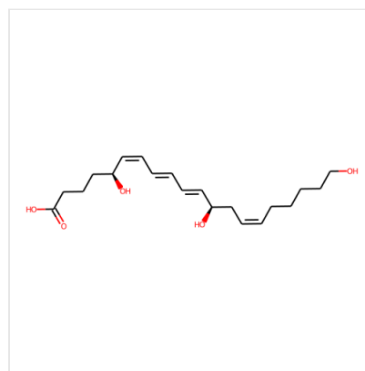
Structure 20-hydroxy Leukotriene B4, CAS 79516-82-8
