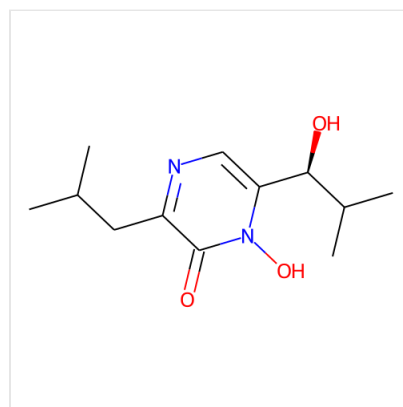
Structure Neohydroxyaspergillilic Acid, CAS 72598-34-6
