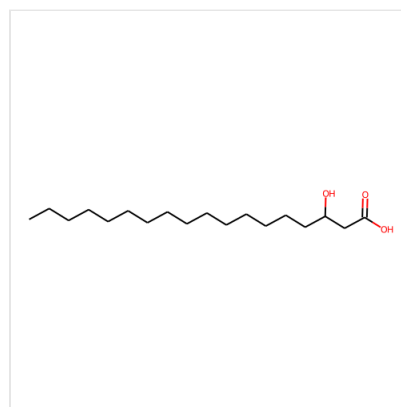
Structure 3-hydroxy Stearic Acid, CAS 17773-30-7
