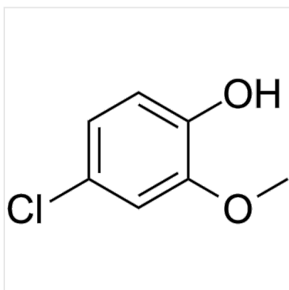
Structure 4-Chloroguaiacol, CAS 16766-30-6
