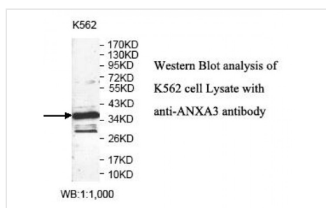
WB (Western Blot) Western Blot analysis of K562 cell Lysate with anti-ANXA3 antibody
