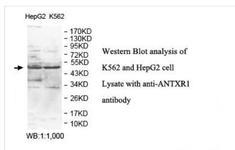
WB (Western Blot) Western Blot Analysis of k562 and HepG2 cell Lysate with ant-antxri antibody
