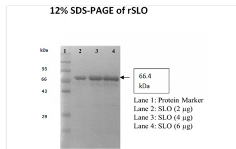
SDS-PAGE Major Band of Streptolysin O is observed at 66.4 kDa
