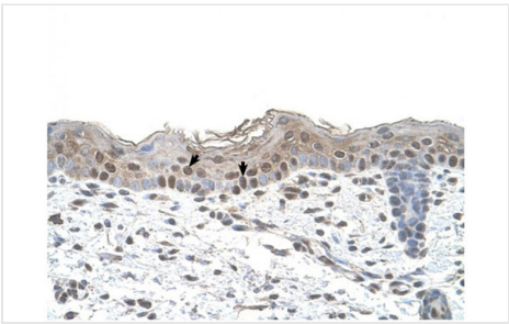
IHC (Immunohistochemistry) Arrestin B2 antibody was used for immunohistochemistry at a concentration of 4-8 ug/ml to stain Squamous epithelial cells (arrows) in Human Skin. Magnification is at 400X
