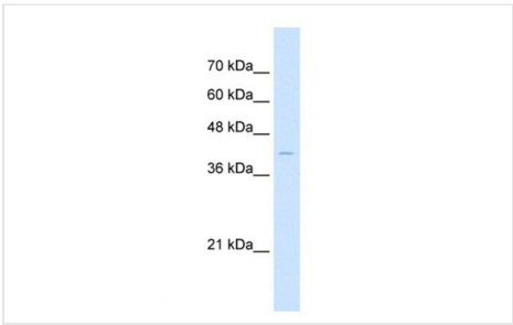
WB (Western Blot) Western Blot showing Arrestin B2 antibody used at a concentration of 1 ug/ml against HepG2 Cell Lysate
