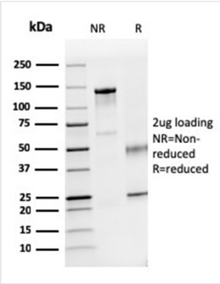
SDS-PAGE SDS-PAGE Analysis Purified Dystrophin Monospecific Mouse Monoclonal Antibody (DMD/3241). Confirmation of Purity and Integrity of Antibody.
