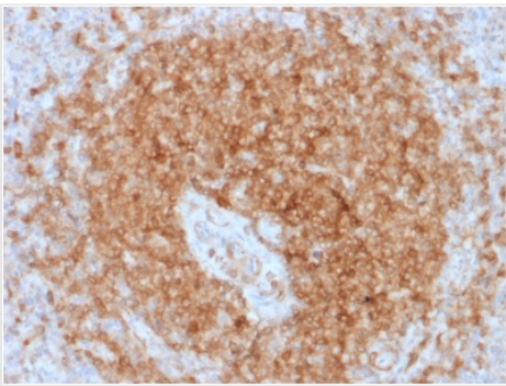
IHC (Immunohistochemistry) Formalin-fixed, paraffin-embedded human Spleen stained with CD79a Mouse Recombinant Monoclonal Antibody (rIGA/764).
