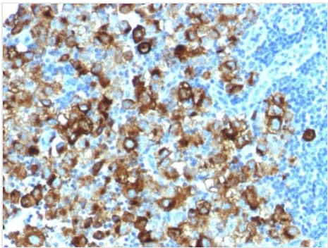
IHC (Immunohistochemistry) Formalin-fixed, paraffin-embedded human Melanoma stained with gp100 Rabbit Recombinant Monoclonal Antibody (PMEL/1825R).
