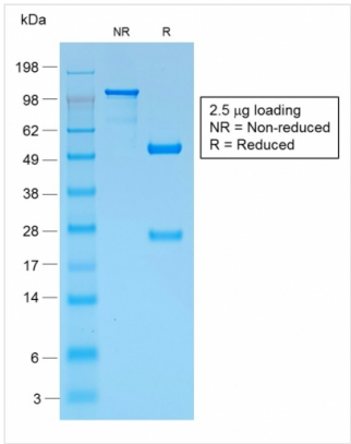
SDS-PAGE SDS-PAGE Analysis Purified gp100 Rabbit Recombinant Monoclonal Antibody (PMEL/1825R).
