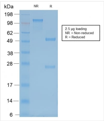
SDS-PAGE SDS-PAGE Analysis of Purified Neurofilament Mouse Recombinant Monoclonal Antibody (rNF421).
