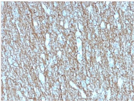
IHC (Immunohistochemistry) Formalin-fixed, paraffin-embedded human Brain stained with Neurofilament Mouse Recombinant Monoclonal Antibody (rNF421).
