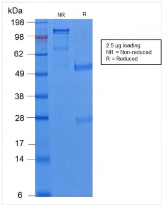
SDS-PAGE SDS-PAGE Analysis of Purified Cytokeratin 8 Rabbit Recombinant Monoclonal Antibody (KRT8/2174R).
