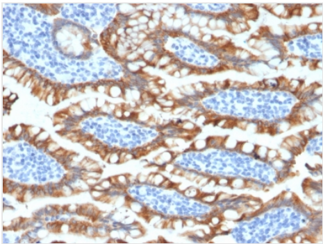
IHC (Immunohistochemistry) Formalin-fixed, paraffin-embedded human Small Intestine stained with Cytokeratin 8 Rabbit Recombinant Monoclonal Antibody (KRT8/2174R).
