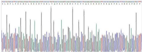
Gene Sequencing (Extract)
