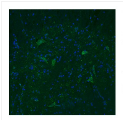
IF (Immunofluorescence) Immunofluorescence: Dilution -- 3ug/mL
