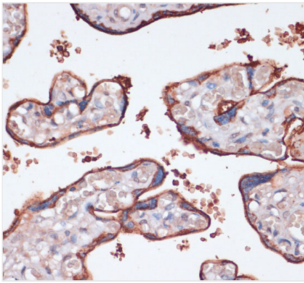
IHC (Immunohistochemistry) Immunohistochemistry of paraffin-embedded Human placenta using RPS6KA2 Polyclonal Antibody at dilution of 1:100 (40x lens).
