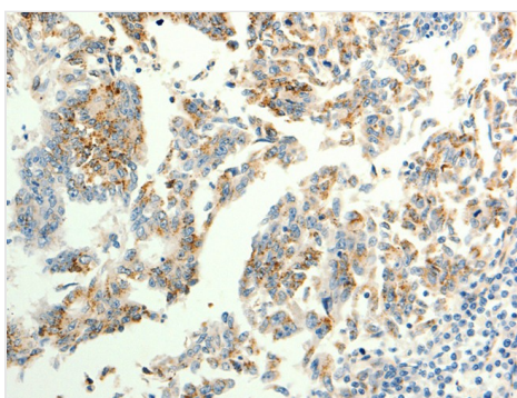
IHC (Immunohistochemistry) Immunohistochemistry of paraffin-embedded Human gastric cancer tissue using TRPC6 Polyclonal Antibody at dilution 1:40
