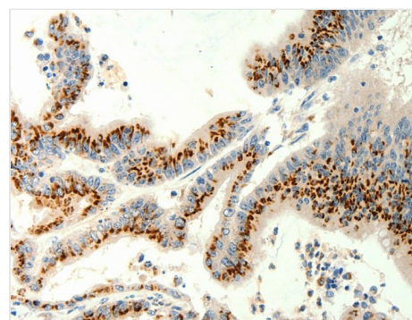
IHC (Immunohistochemistry) Immunohistochemistry of paraffin-embedded Human colon cancer tissue using TRPC6 Polyclonal Antibody at dilution 1:40
