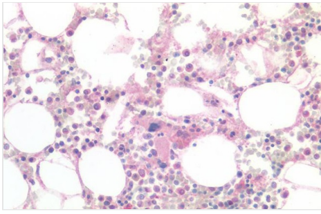
IHC (Immunohistochemistry) MSLN/Mesothelin Antibody-Human Bone Marrow, Megakaryocytes: Formalin-Fixed, Paraffin-Embedded (FFPE)
