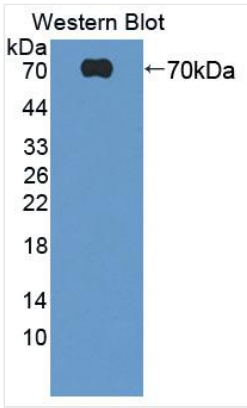
WB (Western Blot) HABP2 Antibody-Western blot of HABP2 antibody.
