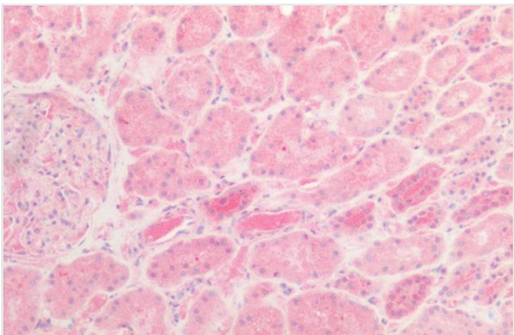
IHC (Immunohistochemisry) HABP2 Antibody-Human Kidney: Formalin-Fixed, Paraffin-Embedded (FFPE)
