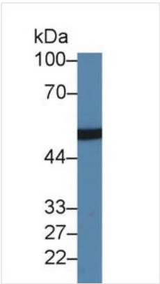
WB (Western Blot) HABP2 Antibody-Western Blot; Sample: Porcine Liver lysate; Primary Ab: 1ug/ml Rabbit Anti-Human HABP2 Antibody Second Ab: 0.2ug/mL HRP-Linked Caprine Anti-Rabbit IgG Polyclonal Antibody
