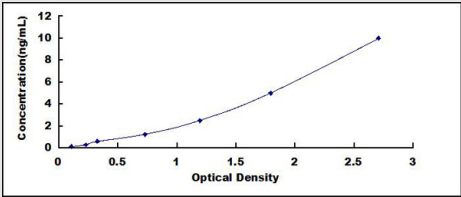
Standard Curve (Sample) Typical Standard Curve for ENPP3 ELISA (Sandwich)
