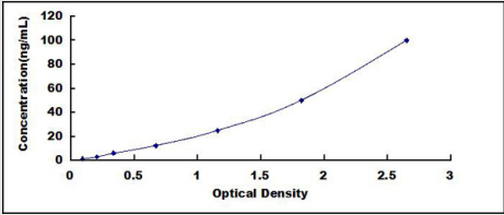
Standard Curve (Sample) Typical Standard Curve for ALT ELISA (Sandwich)
