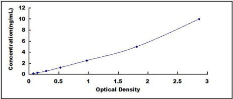
Standard Curve (Sample) Typical Standard Curve for ADC ELISA (Sandwich)
