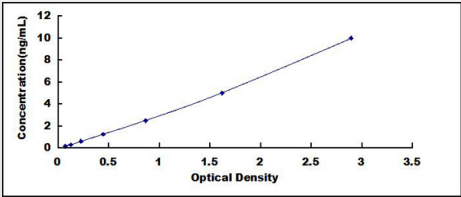
Standard Curve (Sample) Typical Standard Curve for HMGB4 ELISA (Sandwich)
