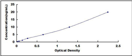
Standard Curve (Sample) Typical Standard Curve for NRCAM ELISA (Sandwich)
