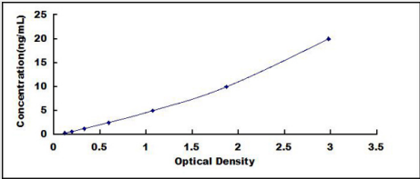
Standard Curve (Sample) Typical Standard Curve for AURKA ELISA (Sandwich)
