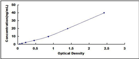
Standard Curve (Sample) Typical Standard Curve for TYR ELISA (Sandwich
