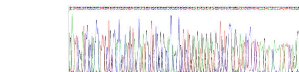
Gene Sequence Gene Sequencing (extract)
