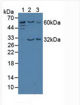
WB (Western Blot) Western Blot: Sample: Lane1: Human Jurkat Cells; Lane2: Human HeLa Cells; Lane3: Human K562 Cells.
