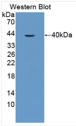
WB (Western Blot) Western Blot: Sample: Recombinant TERF2, Human.
