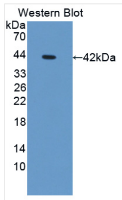
WB (Western Blot) Western Blot; Sample: Recombinant OSTN, Mouse.
